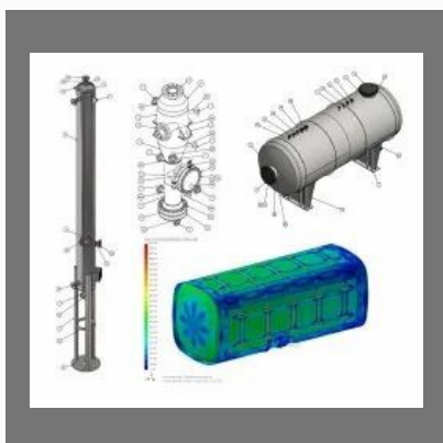
Pressure vessel tank design
