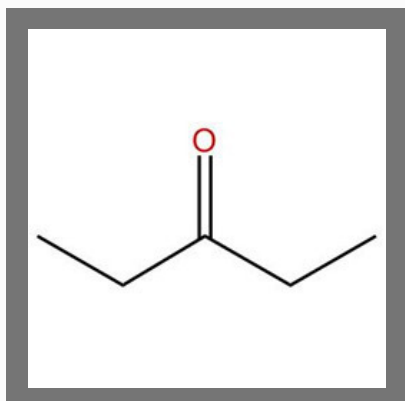
Diethyl Ketone
