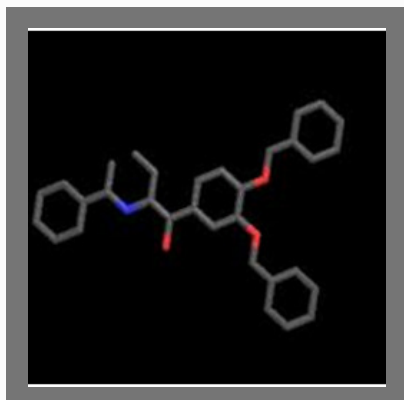
4-Phenyl-1-Butanol
