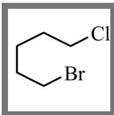
1-Bromo-5-Chloropentane
