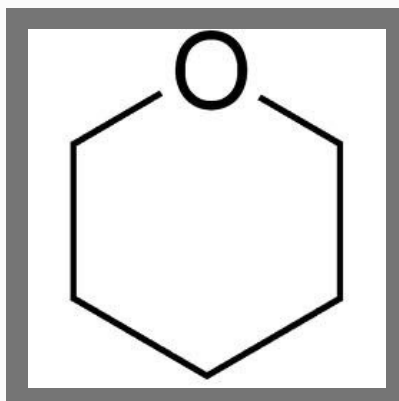
Tetrahydropyran
