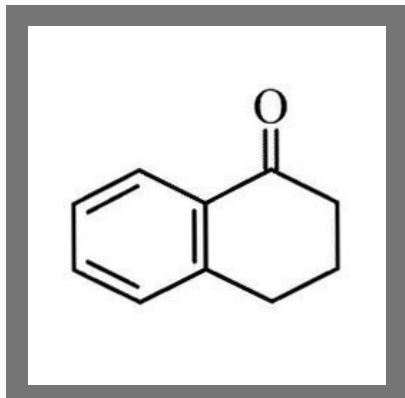
Alpha Tetralone
