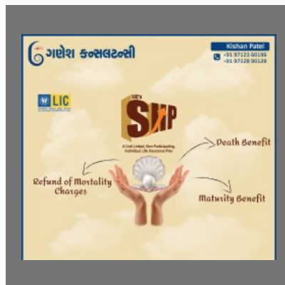
LIC Agent
