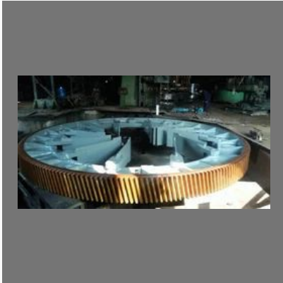
Girth Gears
