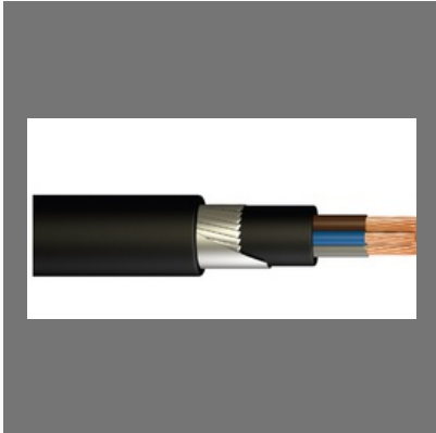
XLPE STA Three Core Cable 12 to 20 KV
