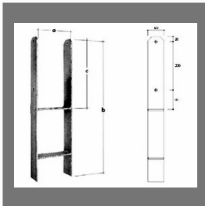
H-type Post Foot / Post Support
