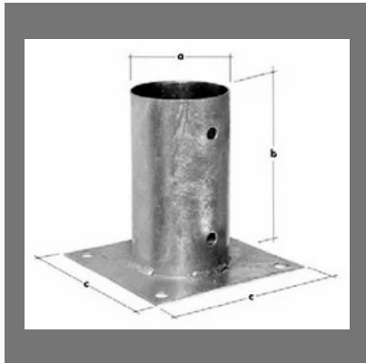
Circular Post Foot / Ground Plate
