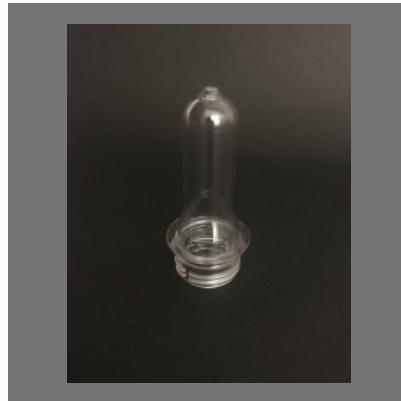
14.2 Gram 1881 PCO PET Preform
