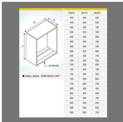
Wall Aqua-gtpt
