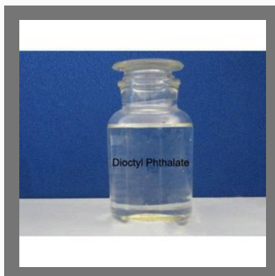
Diocyl-Phthalate
