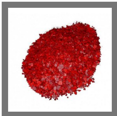
Chromic-Acid
