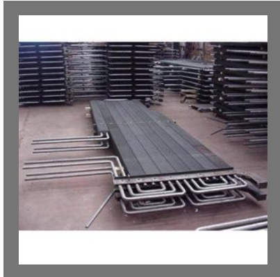
Steel H Power Station Economiser
