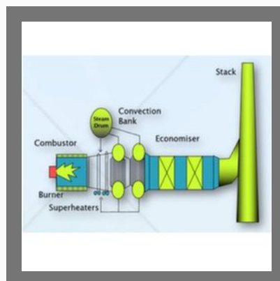
Tail Lean Gas WHR
