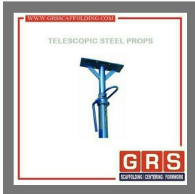
Adjustable Prop Centering
