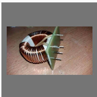
Toroidal Choke
