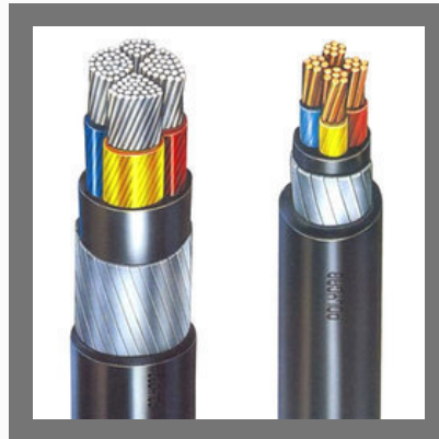
HT and LT Armoured Cables
