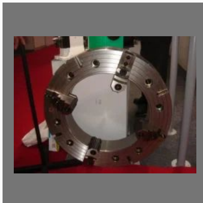
Seco Special Extra Large Bore Chuck
