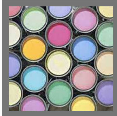
Stoving Paint
