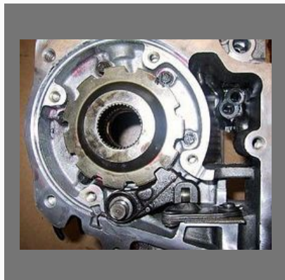
Parking Gear
