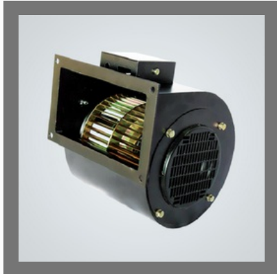
Double Inlet Centrifugal Blower - 450 m 3 /hr - 265 CFM (Model DI133-4E-S2)
