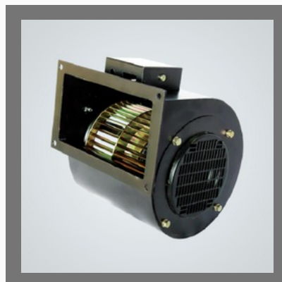
Double Inlet Centrifugal Blower - 1700 m 3 /hr - 1000 CFM (Model DI180-4E-K3)
