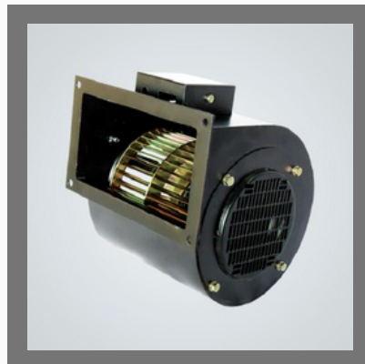
Double Inlet Centrifugal Blower - 1200 m 3 /hr - 705 CFM (Model DI160-2E-S8)
