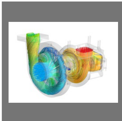
CFD Analysis
