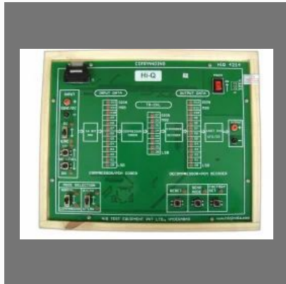
COMPANDING KIT HIQ-4214
