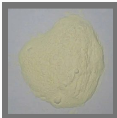
Emamectin Benzoate
