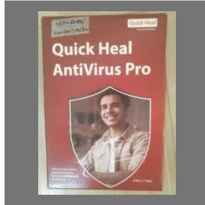
Antivirus
