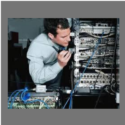
Server Configuration
