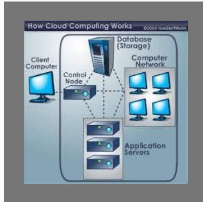
Cloud Computing
