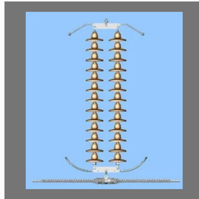
Double Suspension
