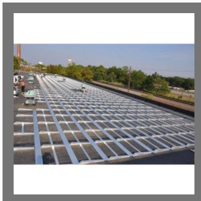
4 mm Solar Panel Mounting Structure
