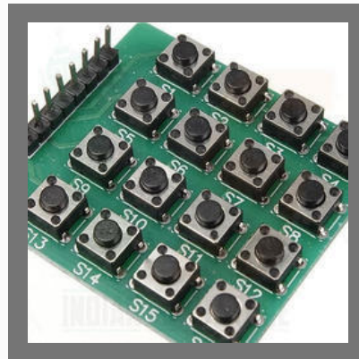
Matrix Keypad Keyboard Module
