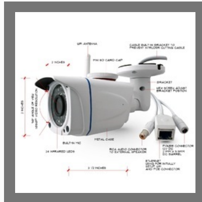
Network IP Bullet Camera
