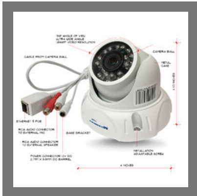
Network IP Dome Camera
