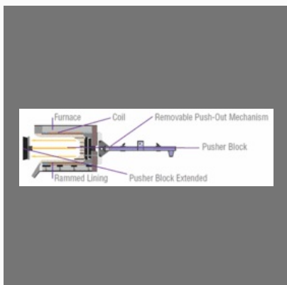
Lining Push-Out Systems For Steel Shell
