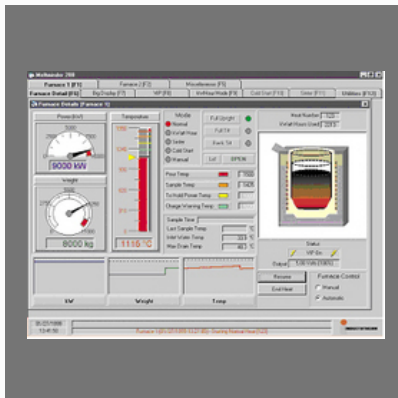
Meltminder Control Systems
