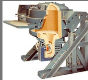
Channel Holding Furnaces
