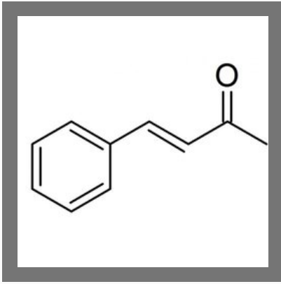
Benzylidene Acetone
