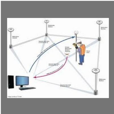
RTK SURVEY
