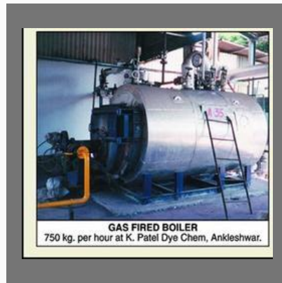
Reverse Flame Gas Fired Boilers-750 Kg Per Hour
