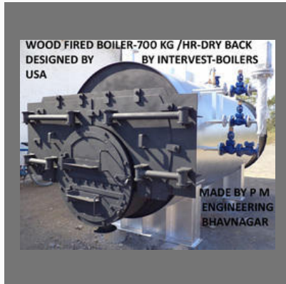
Horizontal Flue Tube Boilers-700 Kg Per Hour
