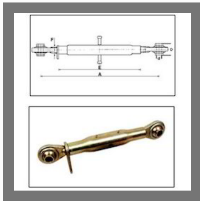
Standard Top - Links Zink Plated
