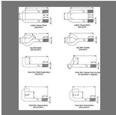
Bent Bolts
