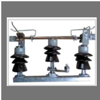
11KV Electrical Isolator
