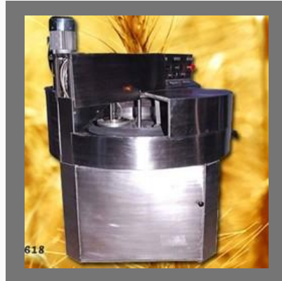
Chapati Machine
