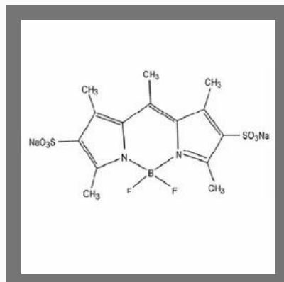
Pyrromethene 546
