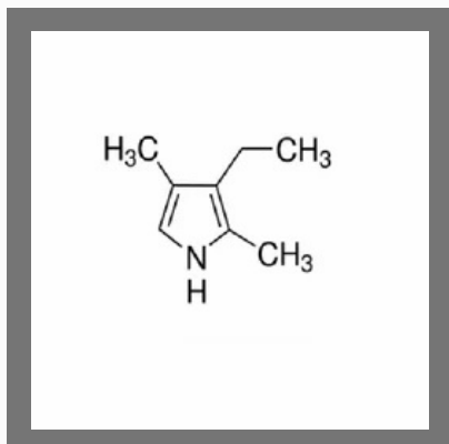
Kryptopyrrole Chemicals
