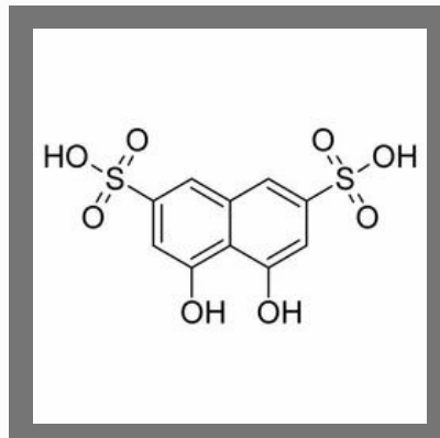
Chromotropic Acid
