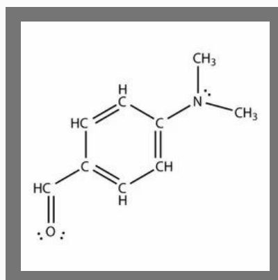
4 Dimethylaminobenzaldehyde
