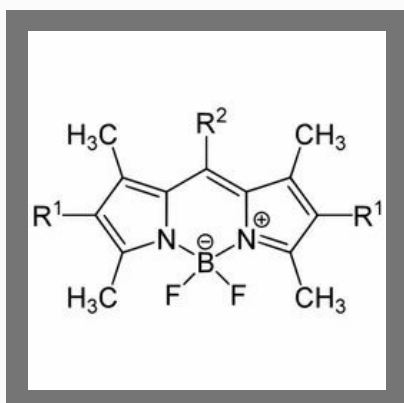
Pyromethene -567
