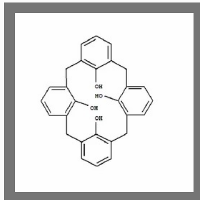
Calix 4 Arene
