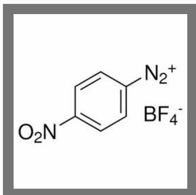
4-Nitrobenzenediazonium Tetrafluoroborate
