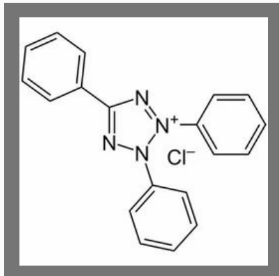
Tetrazolium Red
