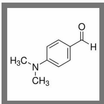
Para Dimethylaminobenzaldehyde
