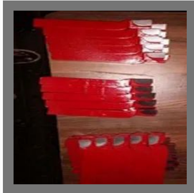
Carbide Brazed Lathe Cutting Tool
