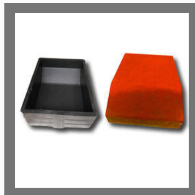
Kerb Stone 2 Paver Blocks Rubber Mould
