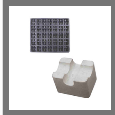
Cover Blocks-1 Rubber Moulds
