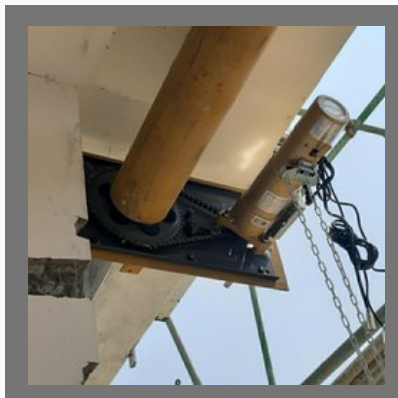
Automatic Rolling Shutters
