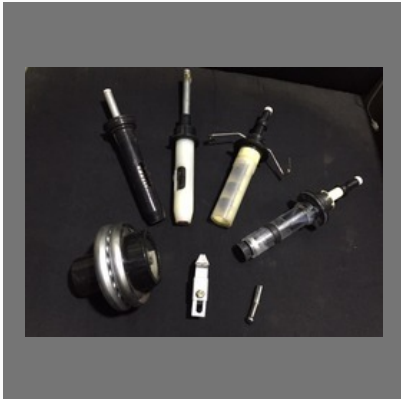
Cotton Tfo Machine All Type Of Tension Devices & Overfeed
