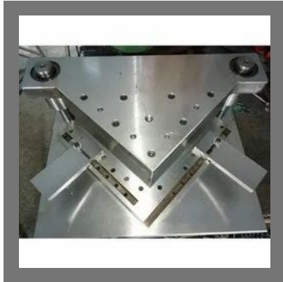
Mild Steel Cutting Die
