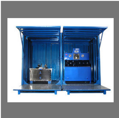
Containerized Offshore Systems
