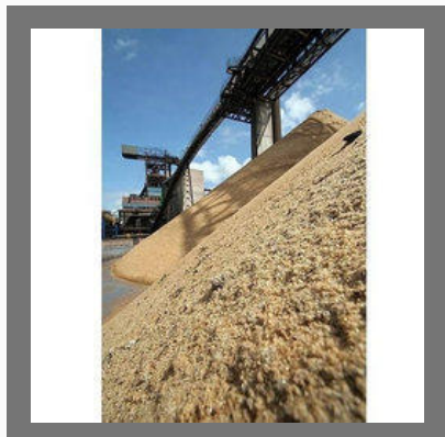
Granulated Blast Furnace Slag
