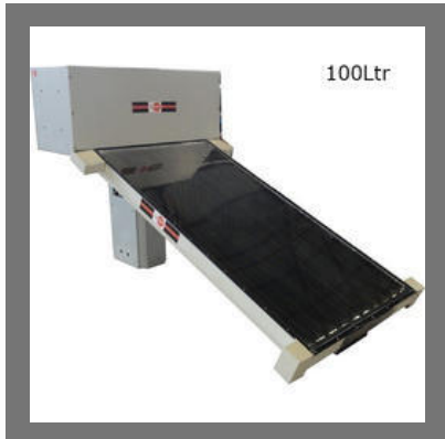
100L Solar Hybrid Heat Pump
