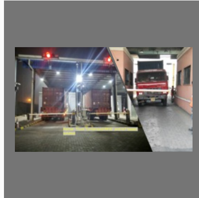
Truck Turnaround System RFID and IOT
