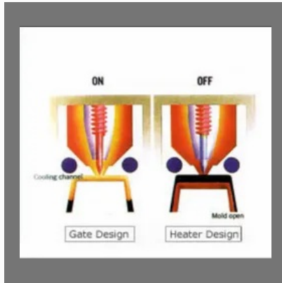
Tip Heater
