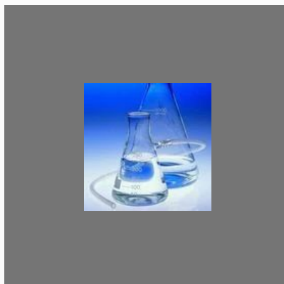
Acetyl Chloride For Synthesis
