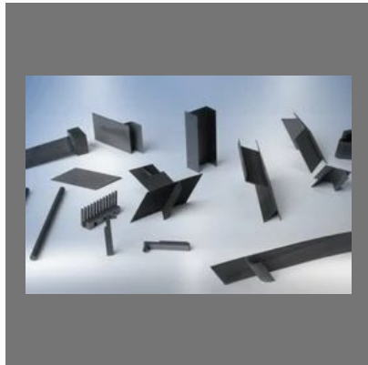
Graphite EDM Electrodes
