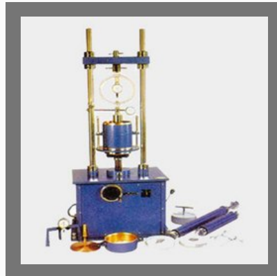
CBR Test Apparatus Motorised Single Speed
