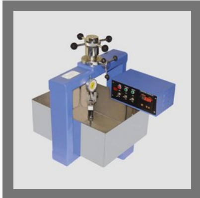
Mastic Asphalt Hardness Tester
