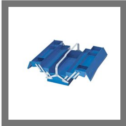
Tool Box
