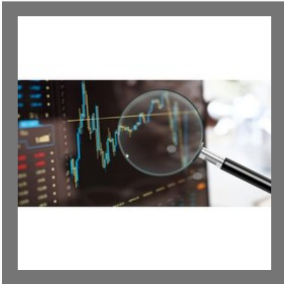
Data Analysis
